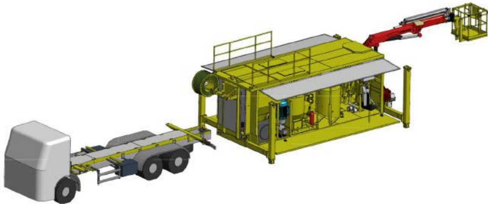
3D-Model of grouting unit with Palfinger crane and AMV basket. Serial NO. 5-10327
